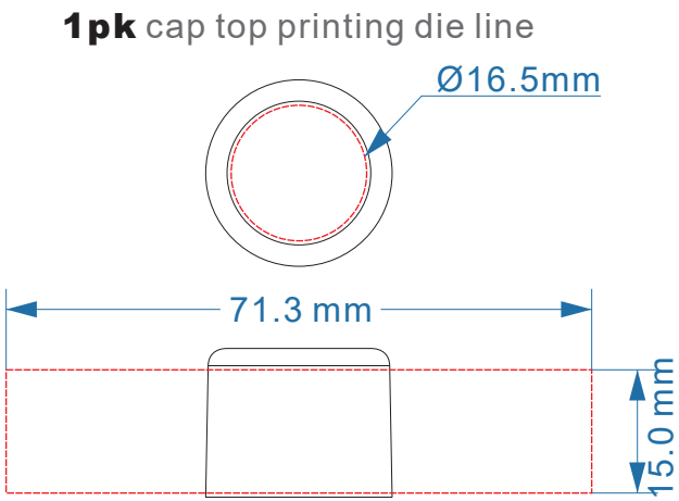
1pk cap side printing die line
