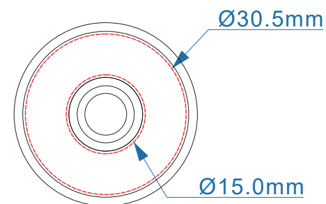
2ml cap top printing die line
